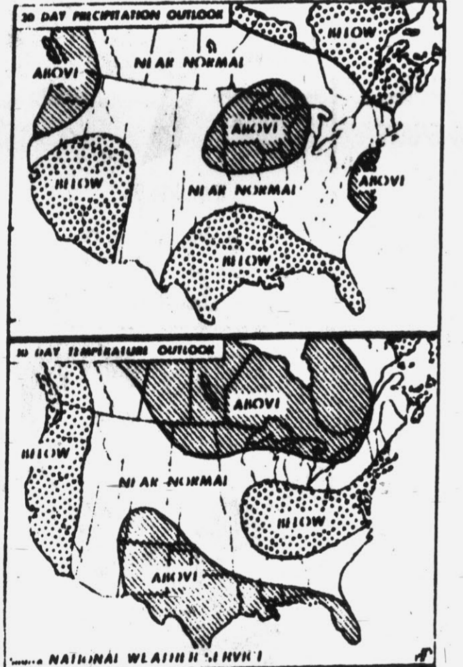
WEATHER OUTLOOK — Maps denote National Weather Service forecasts for the upcoming 30-day period in terms of temperature and precipitation. (AP Wirephoto Map)
