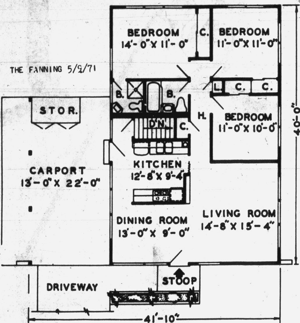
COMFORTABLE AND ECONOMICAL —The Fanning, designed by the Associated Architects, is a handsome three-bedroom contemporary ranch which features economical construction.
