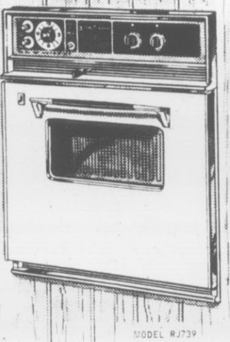
Hotpoint SELF-CLEAN BUILT-IN OVEN WITH ROTISSERIE MODEL RJ739
