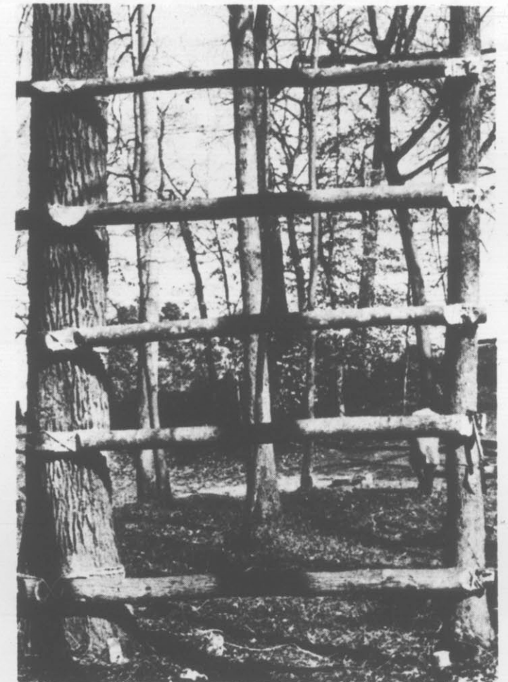
THE IN AND OUT OBSTACLE . . . stresses twisting body movements as a climber weaves in and out. Logs are lashed to the trees to prevent damage which nails or spikes would inflict on the trees.
