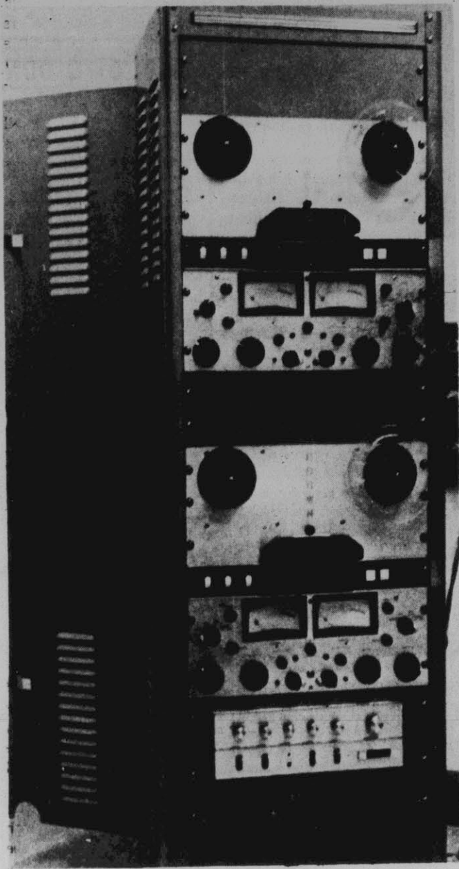
CROWN TAPE DECKS . . . are used to record recitals and for certain stages in electronic music composition.
