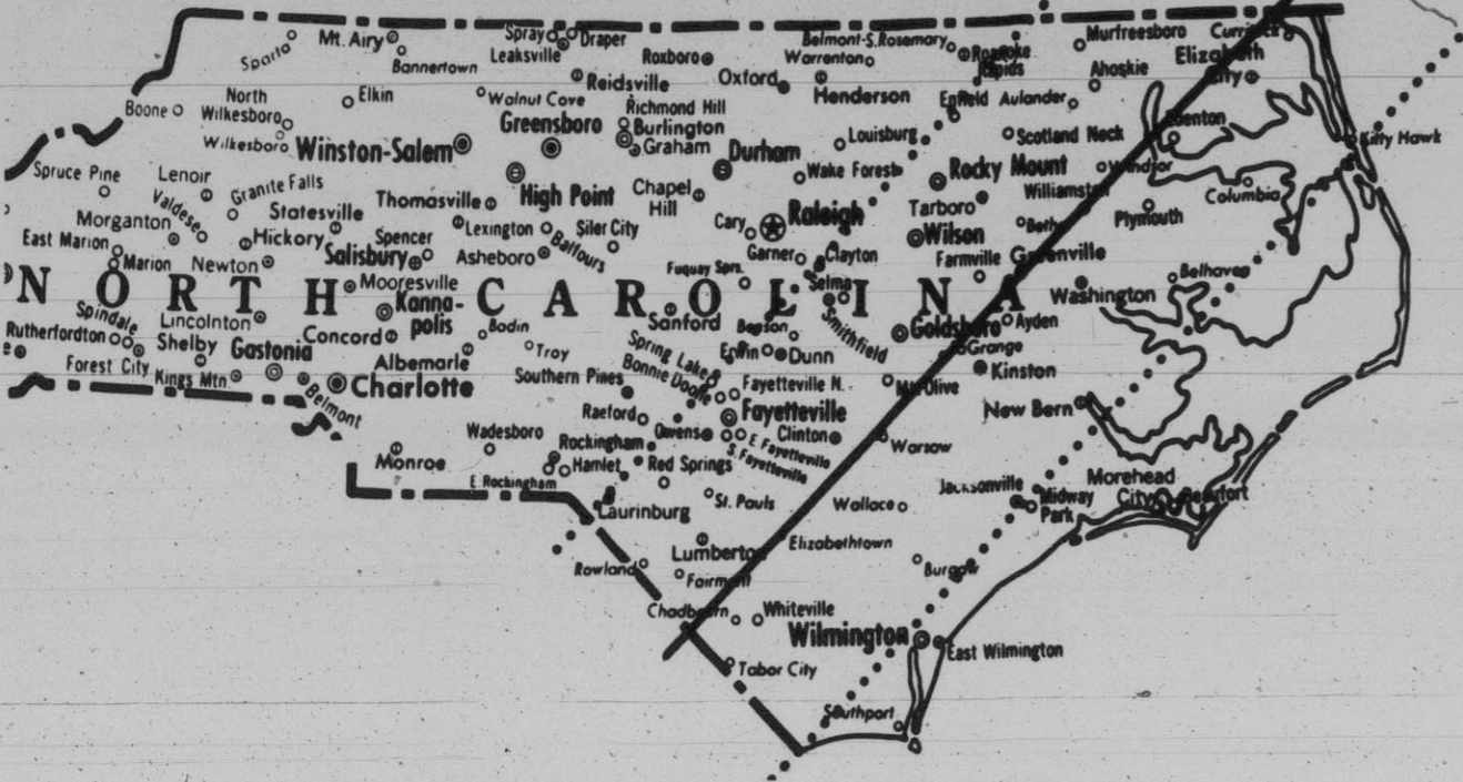
DARK LINE indicates path of the blackout due to solar eclipse.
