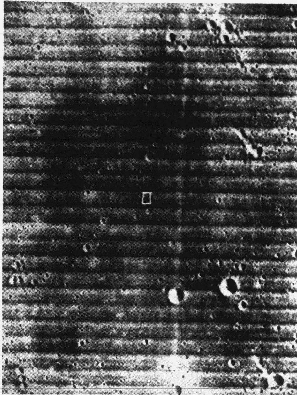
TARGET AREA — This NASA photo shows the specific target area where the Apollo 12 lunar module is scheduled to land in the Ocean of Storms on the western face of the moon. Spacecraft is scheduled to land within about 1,000 feet of the robot spacecraft, Surveyor 3 (small square). (AP Wirephoto)
