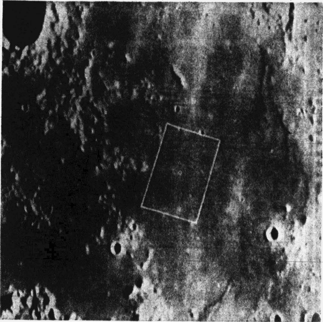
TARGET AREA — This photo shows the general target area where the Apollo 12 lunar module is scheduled to land in the Ocean of Storms on the western face of the moon. The spacecraft is scheduled to land within about 1,000 feet of the robot spacecraft, Surveyor 3 (small circle). The large square indicates area covered by accompanying photo. This picture was taken for NASA by the University of Arizona Lunar and Planetary Laboratory. (AP Wirephoto)
