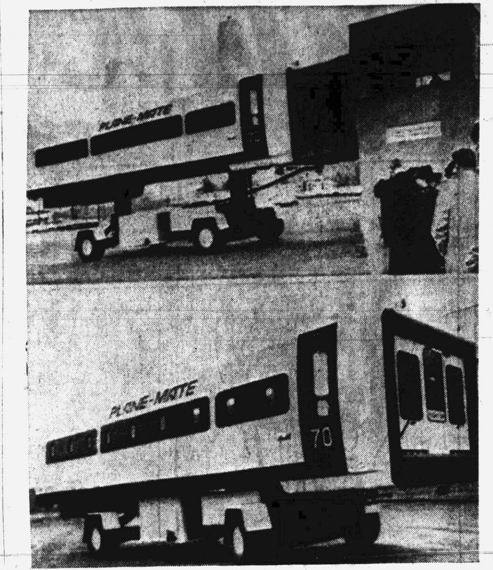
PLANE-MATE UNVEILED — A luxury vehicle designed to load and unload jet plane passengers at congested airports is displayed by its builders, the Budd Company, at Fort Washington, Pa. The carrier can carry up to 150 passengers between terminals and airliners and eliminates step-climbing by elevating the passenger lounge to door of jumbo jets with cabin doors more than 15 feet above the ground. Demonstration shows passengers boarding in its raised position with the lowered vehicle driving off. (AP Wirephoto)
