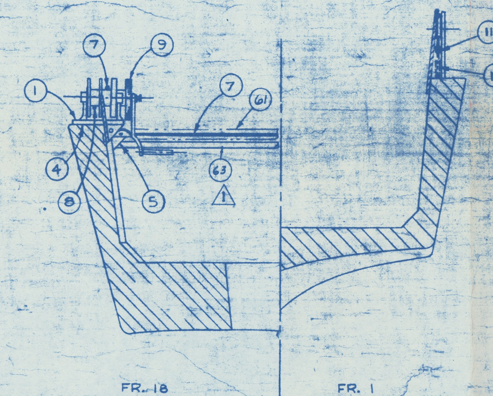
SECTION - LOOKING AFT SCALE: 3/4" = 1'-0"
