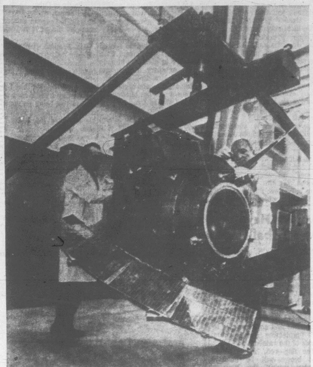
SPIDER-LEGGED SATELLITE CHECKED — Technicians at NASA's Goddard Space Flight Center, Greenbelt, Md., conduct stability check on flight model of the Radio Astronomy Explorer-A satellite, suspended from test stand. The 417-pound spacecraft, designed to study radio emissions, is to be launched July 3 from Lompoc, Calif., test range. Once in orbit four 750-foot antenna booms are to extend from the satellite. (NASA Photo via AP Wirephoto)
