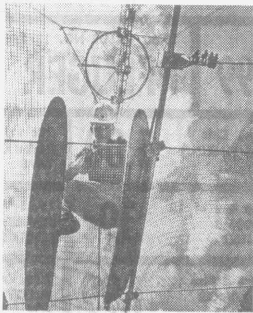
To properly maintain the curvature of the half-inch square wire mesh reflector, workmen move over its surface on water skis to distribute their weight.
