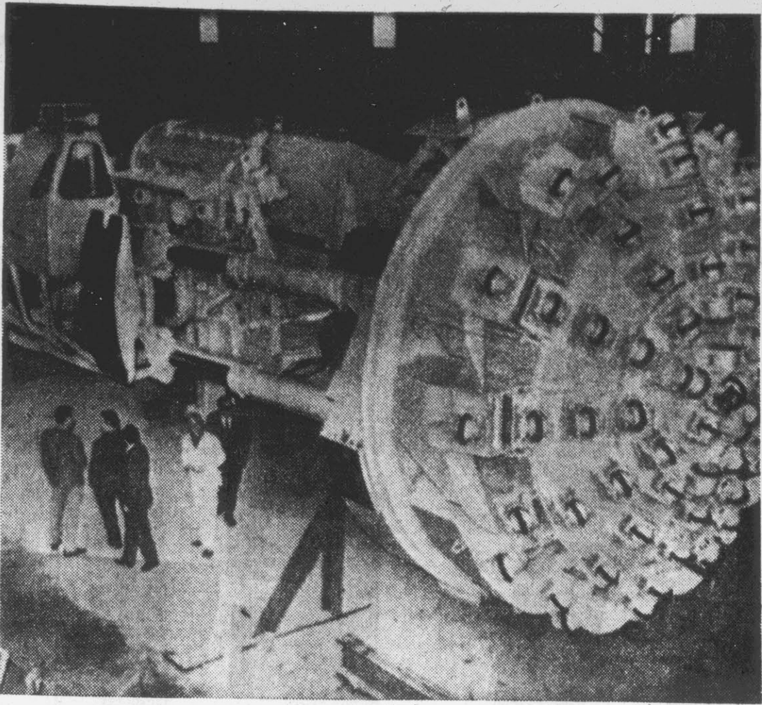
MASSIVE MINING TOOL — This 250-ton hard-rock drilling machine is displayed at Pacific Car & Foundry Co. at Renton, Wash., where it was built for use at White Pine Copper Mine, White Pine, Mich. It will be broken down into 100 parts for shipment and reassembled in mine 2,000 feet underground. Machine's head, right, revolves while 63 bits, each 11 inches in diameter, cut into the rock. (AP Wirephoto)
