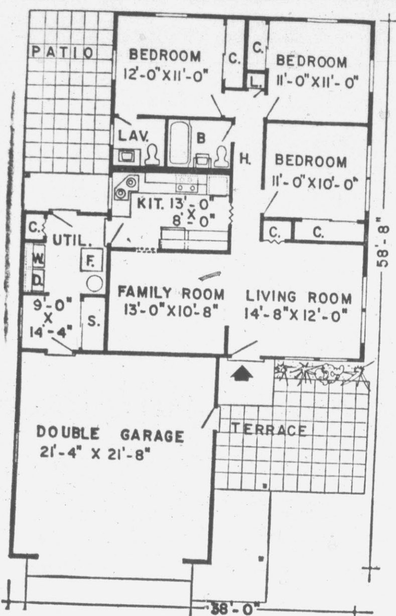
THE SALINA is a ranch-type home, designed for easy living. It's 38-foot width makes it appropriate for most city lots, but it would be attractive on a larger plot in the suburbs, too.
