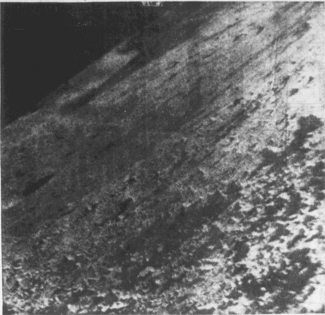
LANDS AMID BOULDERS — This wide-angle (25-degree field of view) picture taken by Surveyor 7 television camera after its moon landing last night shows cluster of rocks near craft's landing site. Scientists said the safe, soft landing amid rocks was by "divine guidance". Horizon, northeast of Surveyor, is formed by ridge characteristic of the undulating topography on the flank of the crater Tycho. Rocky debris, scientists added, was ejected by Tycho some 8 miles to the south. (AP Wirephoto from NASA)
