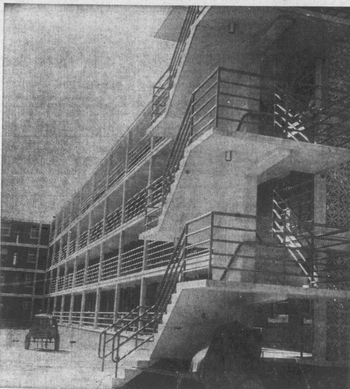
NEARING COMPLETION . . . is East Carolina College's new 500-man dormitory located between 10th and 14th Sts. The new $1,191,000 building is scheduled for completion August 15, in time for occupancy by opening of the Fall term at the college. The four-story dorm includes four-room suites opening to covered outside walkways there-by dispensing with inside halls.
