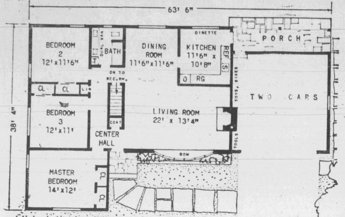
THIS RANCH HOUSE looks a lot larger than its 1,330 square feet. There are three bedrooms and a smart double lavatory bath. The kitchen is at the side rear, with ready access to dining room, porch behind the garage and garage itself. A basement recreation room also is a feature of Plan HA241C. Architect is Lester Cohen, Room 75, 117 W. 48th St., New York 36, N. Y.
