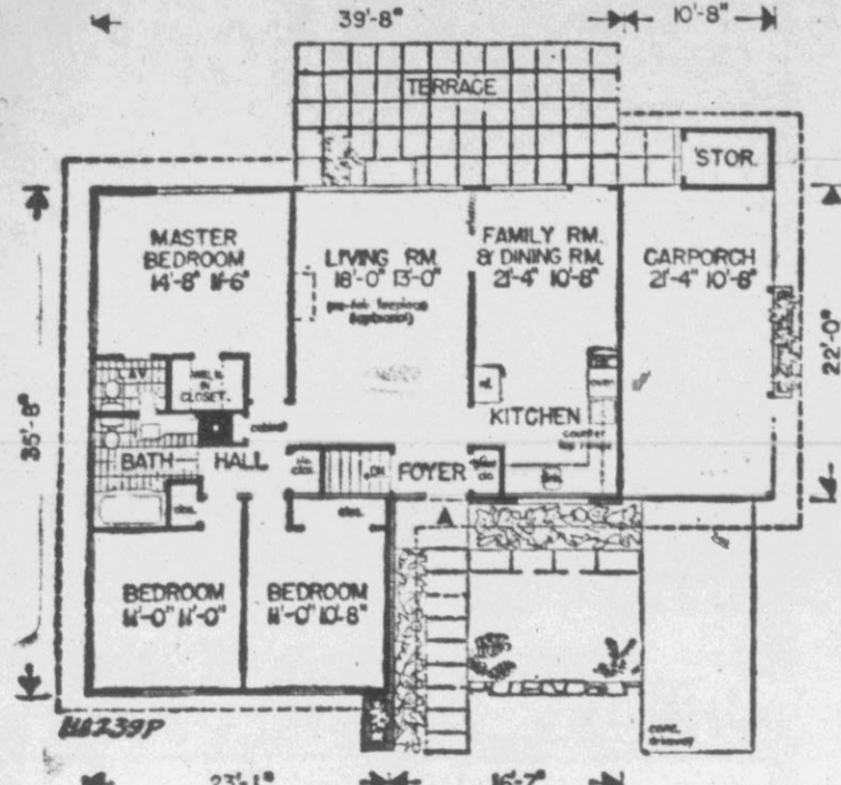
FLOOR PLAN
