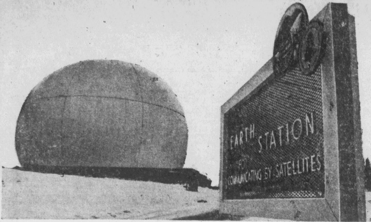
Telstar's ground station, Andover, Me. Huge 340-ton horn antenna has been built inside radome to transmit signals up to satellite and to receive signals from it.
