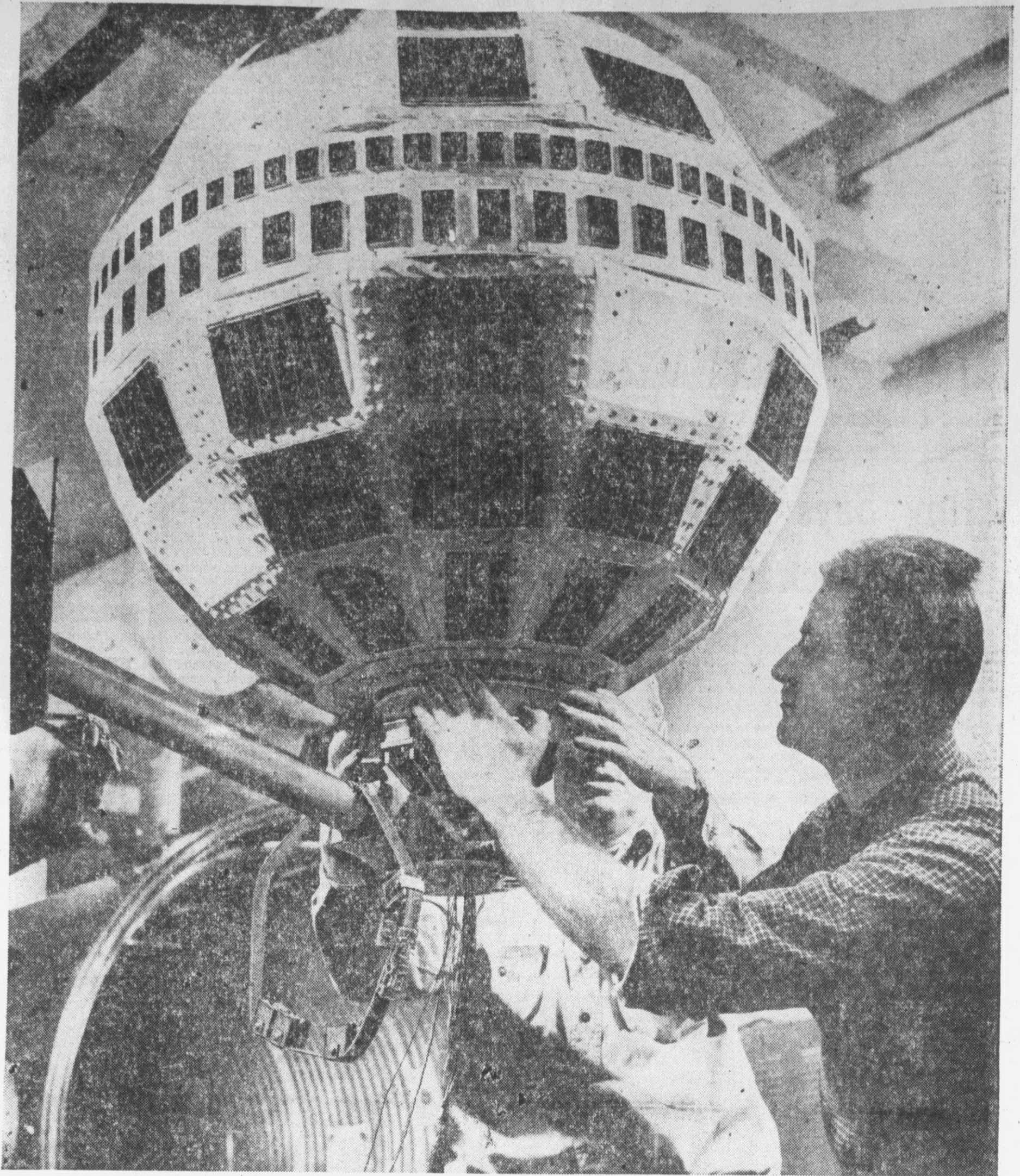
Technicians prepare to give space-simulation test to the Telstar. This model of satellite will be put into vacuum chamber, lower left. Walls of chamber are cooled by liquid nitrogen, simulating heat absorption of space, and chamber will be pumped to a vacuum approximating space. Thermo-couples inside satellite measure temperatures satellite can be expected to attain when it's really in space.
