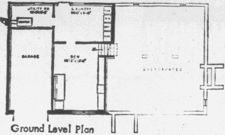
Ground Level Plan
