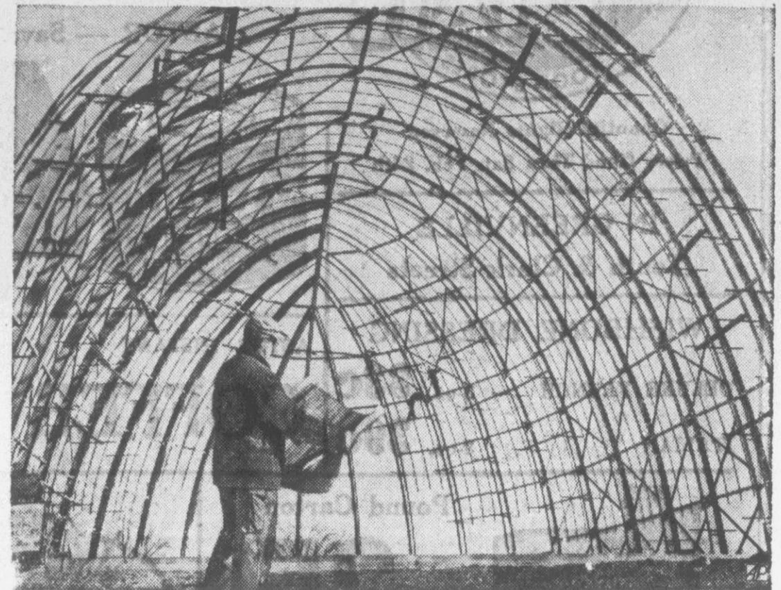
SETTING UP FRAME — Steel structure foreman checks plans as welders piece steel framework for Sacred Heart Roman Catholic church in Waltham, Mass. Building will have circular motif with semi-circular arrangement of pews seating 900 persons.
