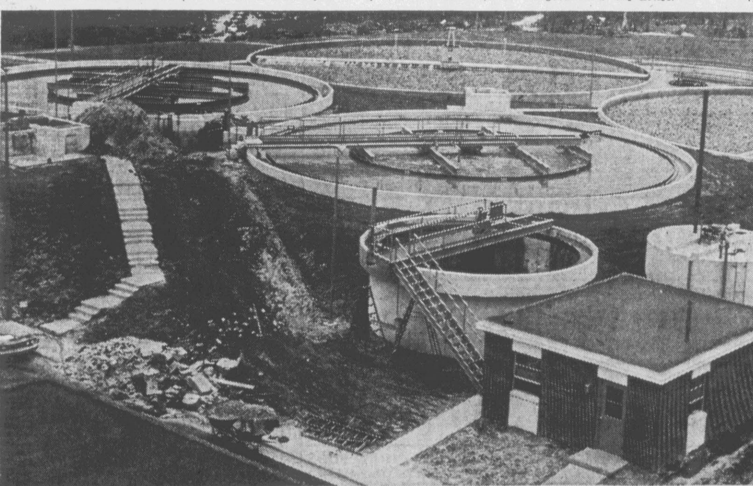
NOW IN OPERATION . . . Greenville's Water Pollution Plant began limited operation yesterday and continued today. Twin circular tanks in center are primary clarifiers while tanks in background are filters. Circular tank near pump building is a secondary clarifier.
