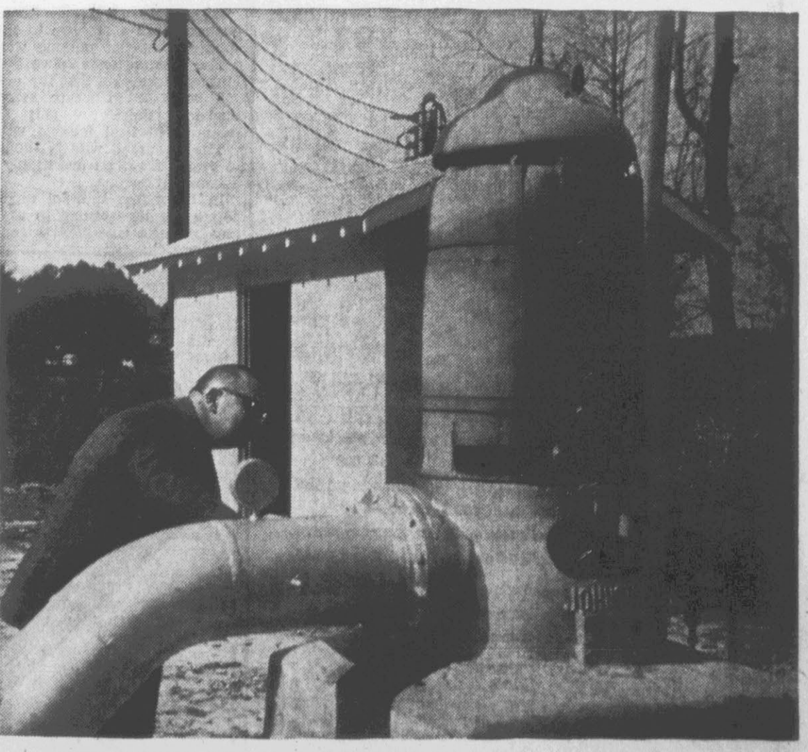
UTILITIES DIRECTOR Leonard Bloxam looks over the pump on the Utilities well at Greenville Blvd. and 14th St. The pump is turned on and off from the Utilities plant by two way radio. Plant operators send a tone over the radio system when additional water is needed in the elevated tanks. As the tanks reach their capacity the pump is turned off by transmission of a signal. (Reflector Staff Photo)
