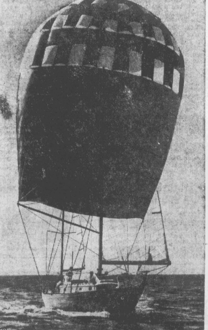
NEW SPINNAKER: The sailmaker who designed this balloon-type sail says the transverse rows of vents speed up the flow of air and greatly reduce knockdown when close reaching. He says it will increase boat speed and that it will be tried on 19-foot lightnings and 33-foot Internationals
