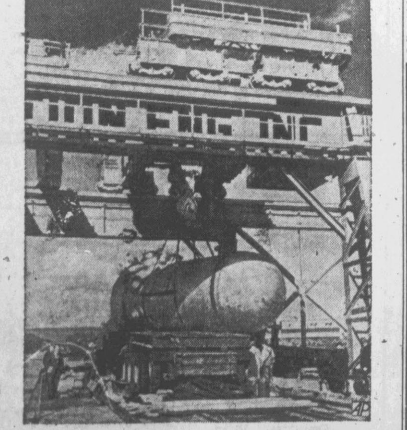
SET FOR TRIP —A 20-ton nuclear reactor vessel is prepared at Chattanooga, Tenn., for shipment to northern Italy for its use in generating electric power.
