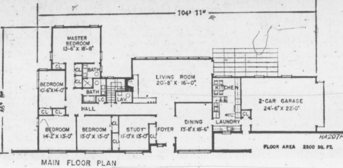
RANCH MANSION: This big ranch-type home with four or five bedrooms has the spaciousness of a mansion. The living room is at the back with a fine terrace adjacent. The architect is Caleb Hornbostel, Room 75, 117 West 48th St., New York 36, N. Y. and the plan is HA207H.
