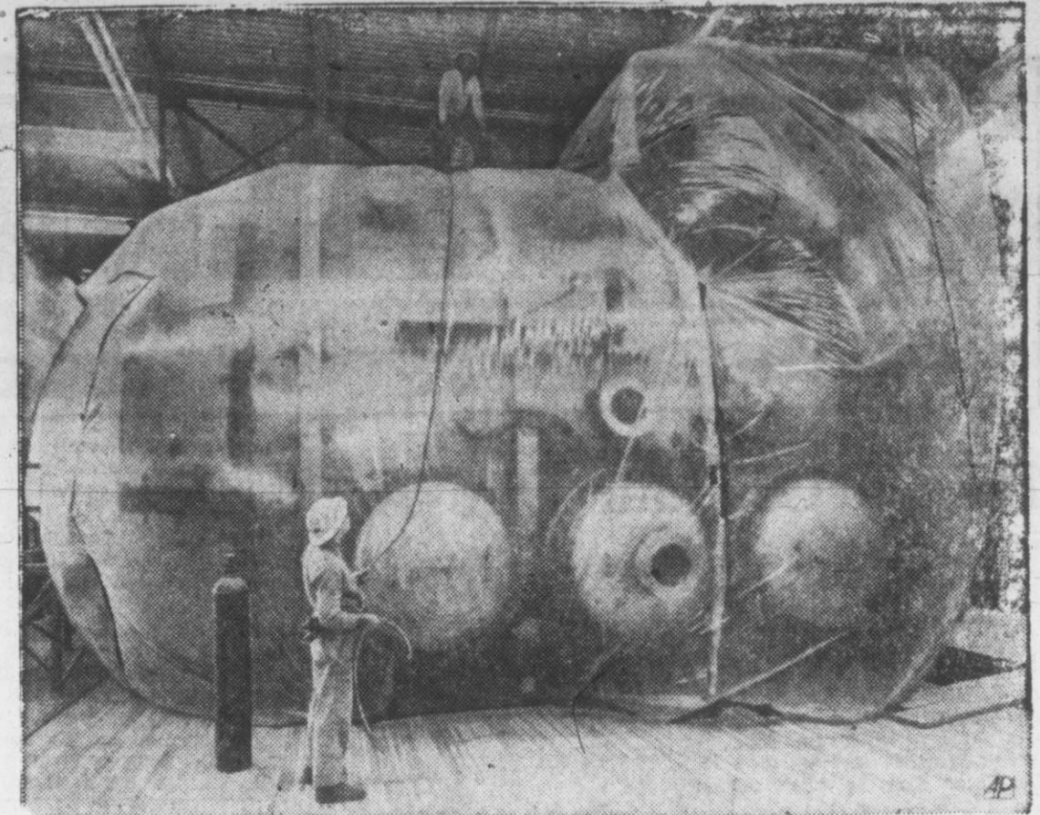
TESTER TESTED — Final checkout of Bendix Corp. chamber for testing space capsules is made at Ann Arbor, Mich. Polyethylene bag filled with helium encloses 20 by 27-foot chamber as it is pumped down to vacuum of space at altitude of over 246 miles.
