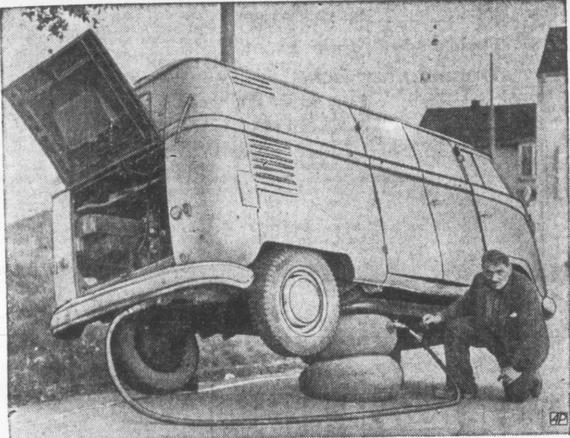
HE SAYS IT'S EASY —Wilhelm Ochs of Kassel, West Germany, shows how he changes tires. He makes a pneumatic jack by using balloon tires inflated by car's exhaust gases. A metal plate is placed between balloon tires and the vehicle's underside.
