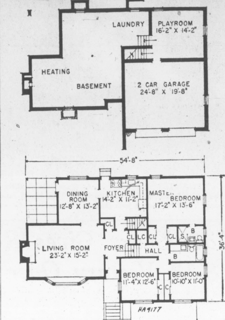
STRIKING SPLIT-LEVEL: A playroom joins laundry and heating space plus a two-car garage in the basement of this split level. The 1,526-square-foot house combines three bedrooms, dining room and kitchen with generous living area. The architect is Caleb Hornbostel, Room 75, 117 W. 48th St., New York 36, N. Y. Plan is HA9177.
