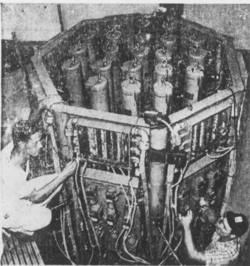
Nuclear testing engineer George Kacer, left, and Howard Veit check control rod drives atop reactor before fueling.
