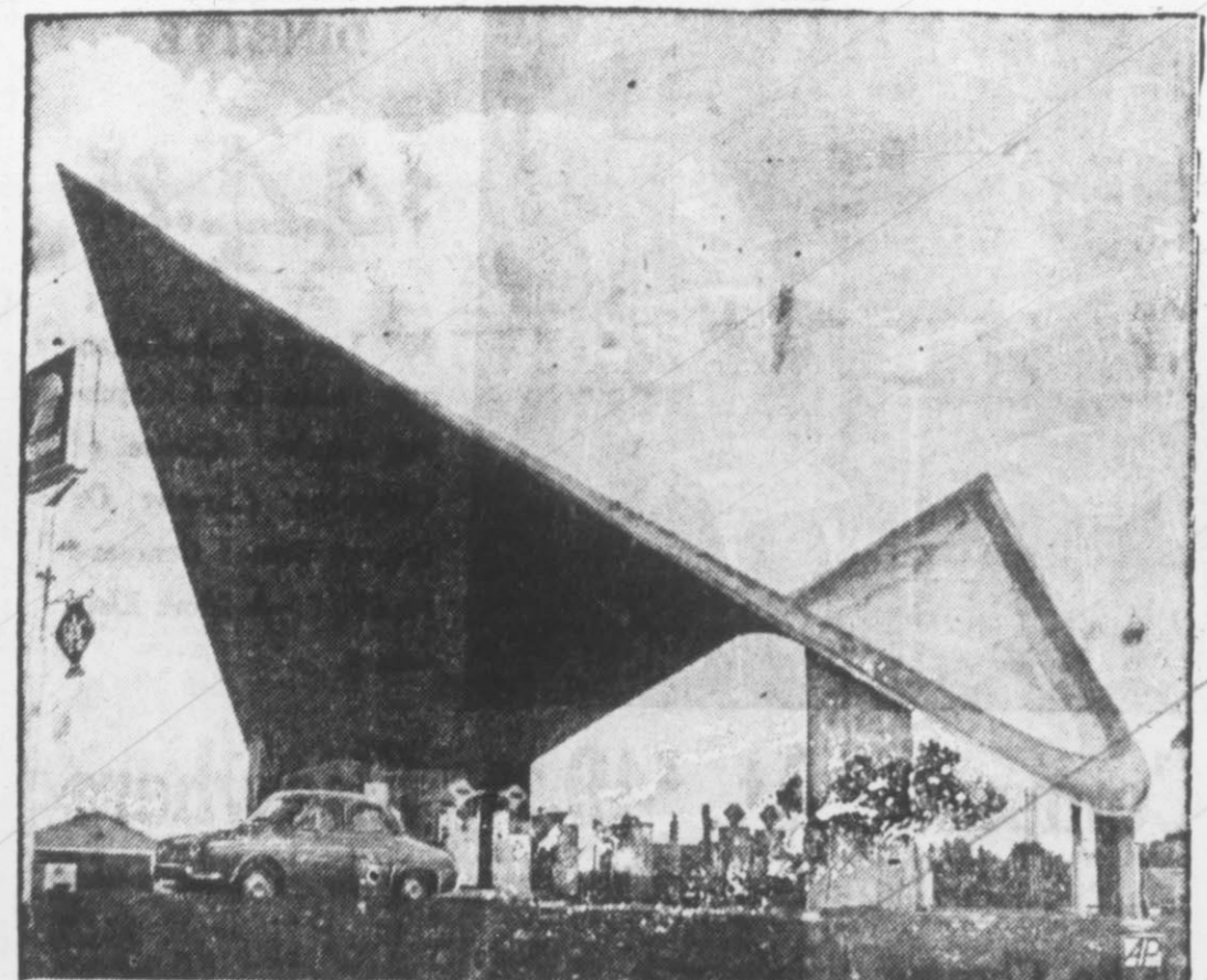
NEW SLANT ON SERVICE—Service station at Retford, England, goes modern with this unusual roof design. Architect calls it a hyperbolic deraboloid structure. It is made of reinforced concrete and weighs about 90 tons. Motel will be added.
