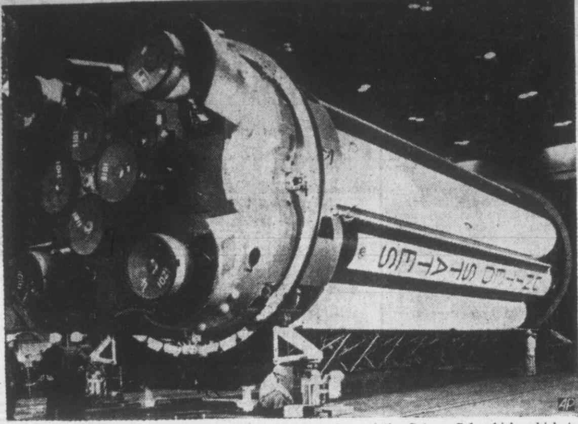
PLENTY OF PRIMARY POWER—This is the first stage of the Saturn C-1 vehicle which is expected to be launched from Cape Canaveral, Fla., this week. The first stage is powered by eight rocket engines. In static tests, 1.3 million pounds of thrust have been developed in firing of the complete Saturn engine. The vehicle is shown in the fabrication and assembly division at NASA's Marshall Space Flight Center, Huntsville, Ala., before it was shipped to Florida. (AP Wirephoto)
