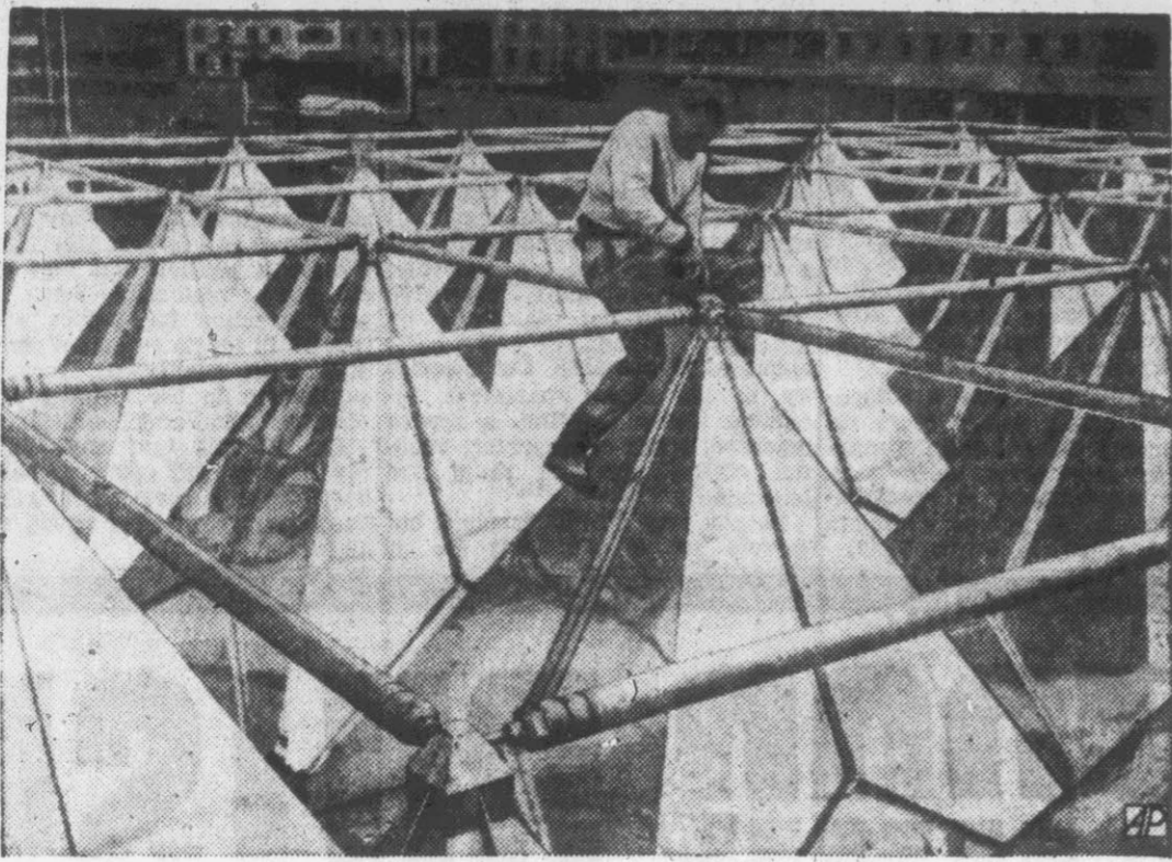
ON TOP OF HIS JOB—A workman checks supporting scaffolding atop unusual roof of building completed in London for international architects' congress. Roof is composed of pyramids or tetrahedrons of aluminum sheet to demonstrate its tensile strength.
