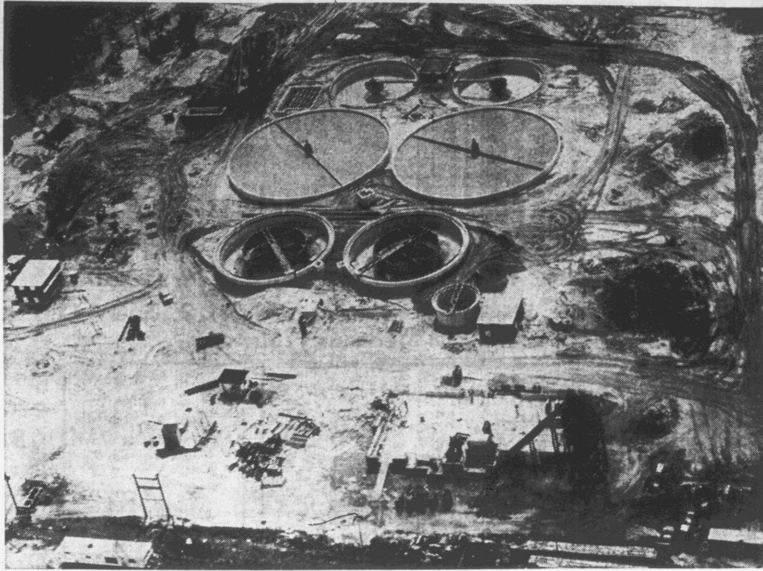
GREENVILLE'S SEWAGE TREATMENT PLANT . . . This air-view shows the local sewage disposal plant, which is about 70 per cent complete. Utilities director Leonard Bloxam said target date for completion is late fall or early winter. The major structures pictured are the pumping station, (brick building at far left); the secondary clarifiers (two large circular structures at top); the trickling filters (circular structures in center); and the primary clarifiers (circular structures at bottom). Also pictured are the control building, which will house the lab, office and storage facilities, (lower right); and the vacuum filter, (tall structure to right of control building).
