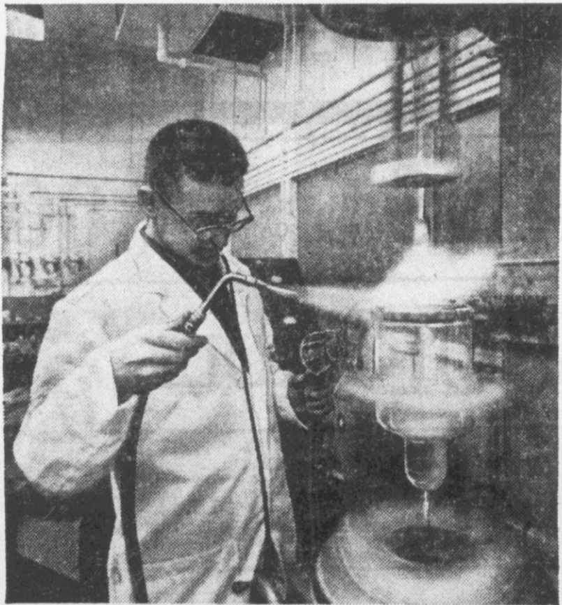
In electron tube shop, glass blower completes final seal on specifically designed electron tube on vertical lathe. He uses extremely hot oxygen-hydrogen flame.
