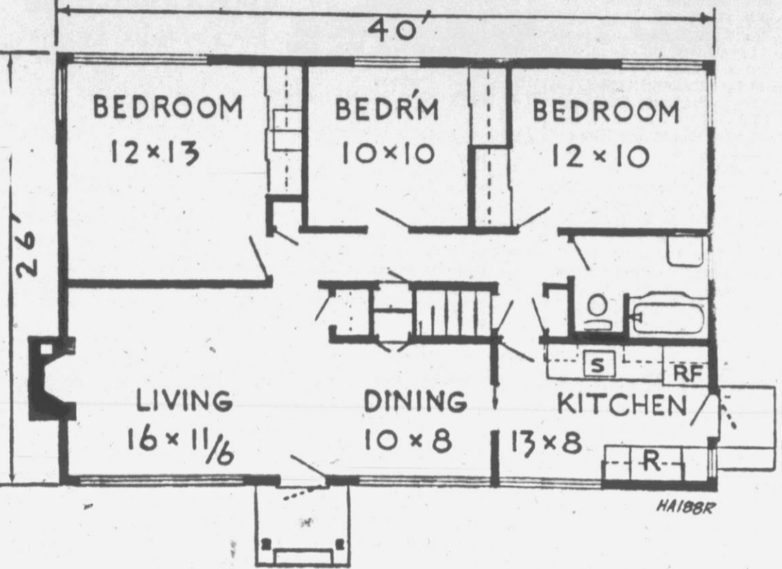
PRIVACY UNLIMITED: All three bedrooms are located in the rear of this one-story frame home, offering the maximum in privacy. Living room, kitchen and dining area line the front. The architect is Jan Retzer, Box 96, New Port Richey, Fla., and the plan is HA1882.
