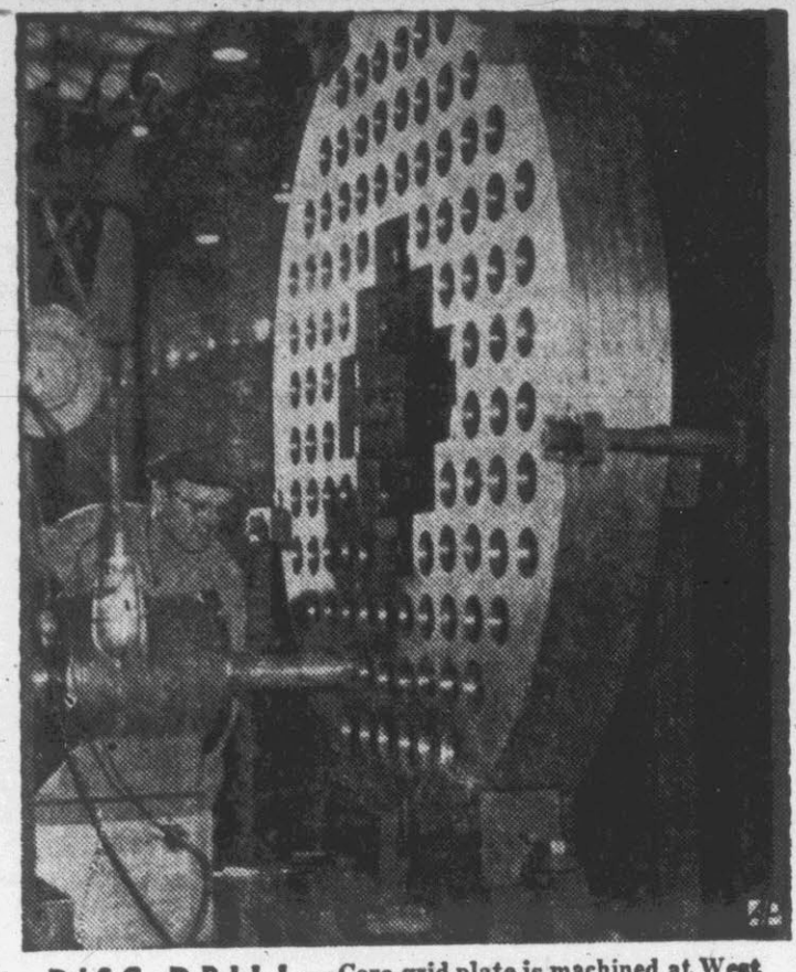
DISC DRILL —Core grid plate is machined at West Allis, Wis., plant. It's for nuclear reactor to be installed at the Pathfinder Atomic Plant near Sioux Falls, S. D.
