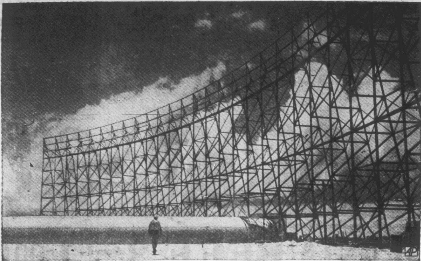
PACIFIC DEFENSE LINK—This is the shielding fence to deplete lethal radio frequency waves generated by transmitter at the Zeus Acquisition Radar (ZAR) center on Kwajalein atoll. Metal tunnel extends from fence to transmitter building.
