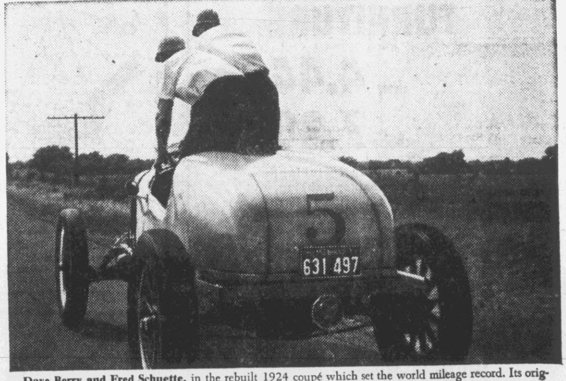
Dave Berry and Fred Schuette, in the rebuilt 1924 coupe which set the world mileage record. Its original frontal area was reduced by about 75 per cent to cut down wind resistance.
