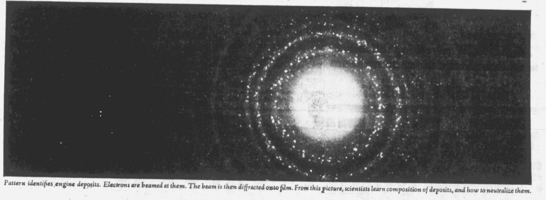
Pattern identifies engine deposits. Electrons are beamed at them. The beam is then diffracted onto film. From this picture, scientists learn composition of deposits, and how to neutralize them.
