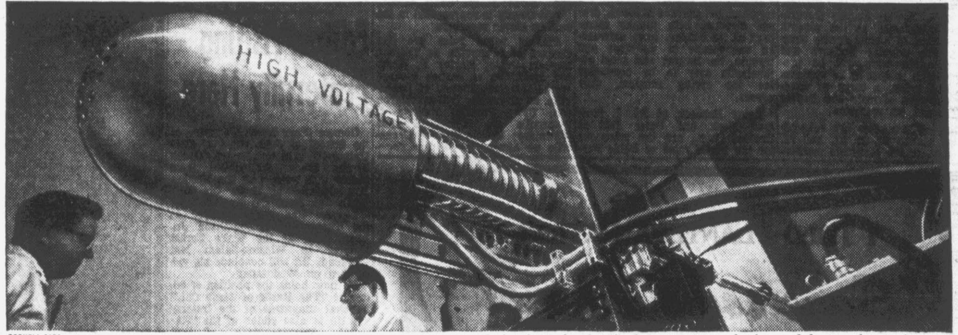
Neutrons generated by this "positive ion accelerator" help Shell scientists make fast chemical analyses for their continuous study of engine behavior and top performance.
