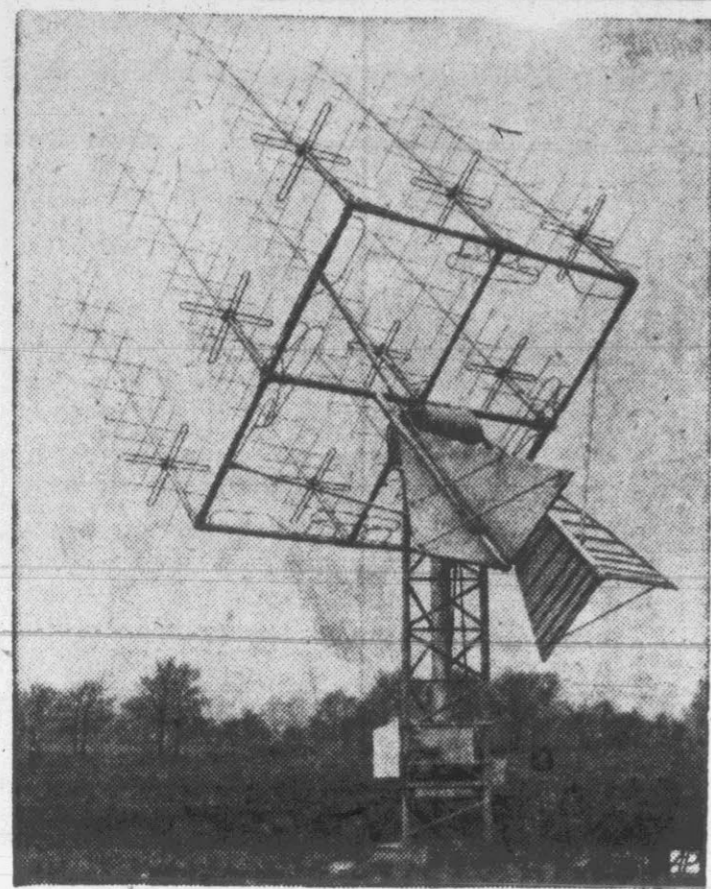
SPACE CHECK — This is one of the remote-controlled rotating aerials set up at Winkfield, Eng., to track U.S. satellites and to follow the first British satellite.
