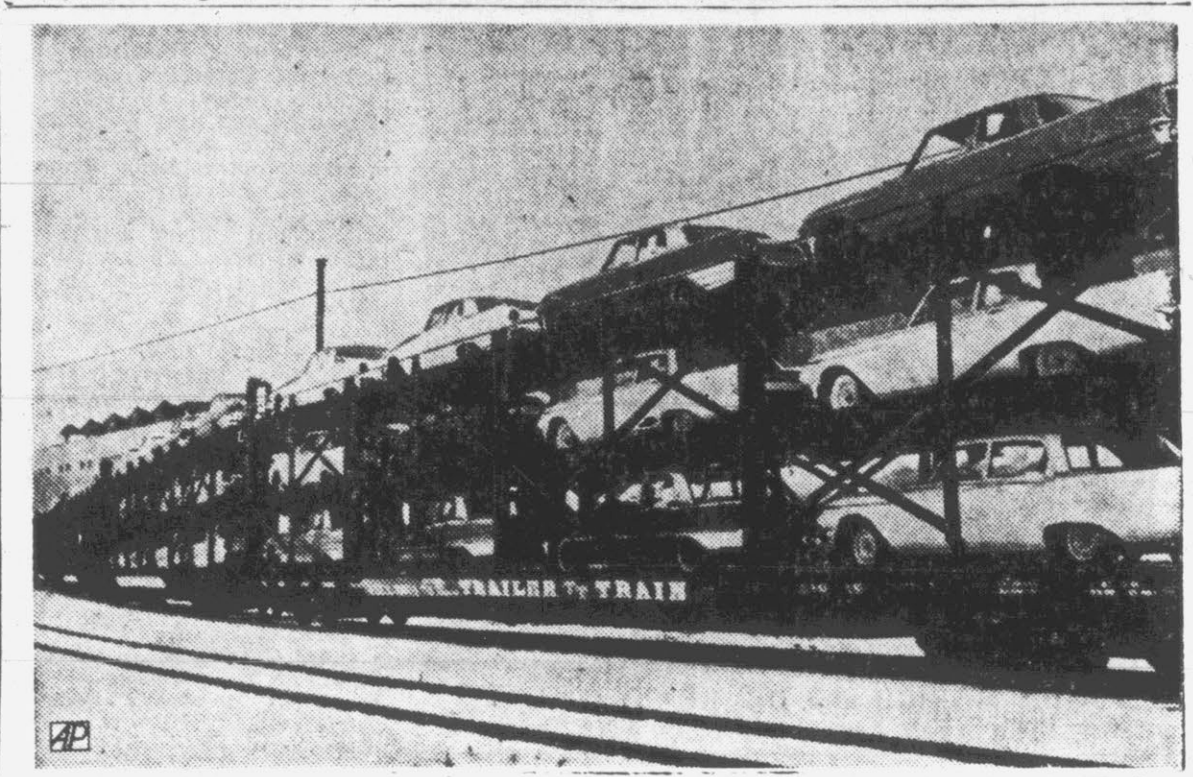
TRAILER TRAIN—Six cars of the Louisville & Nashville Railroad's tri-level "Trailer Train" speed out of Nashville for Memphis where a specially built dock and unloading facilities await. Each flatbed car with its special rack carries 12 regular or 15 "compact" autos from factory to agency. The L&N was among the developers of the Trailer Train which recently went into operation. (AP Wirephoto)
