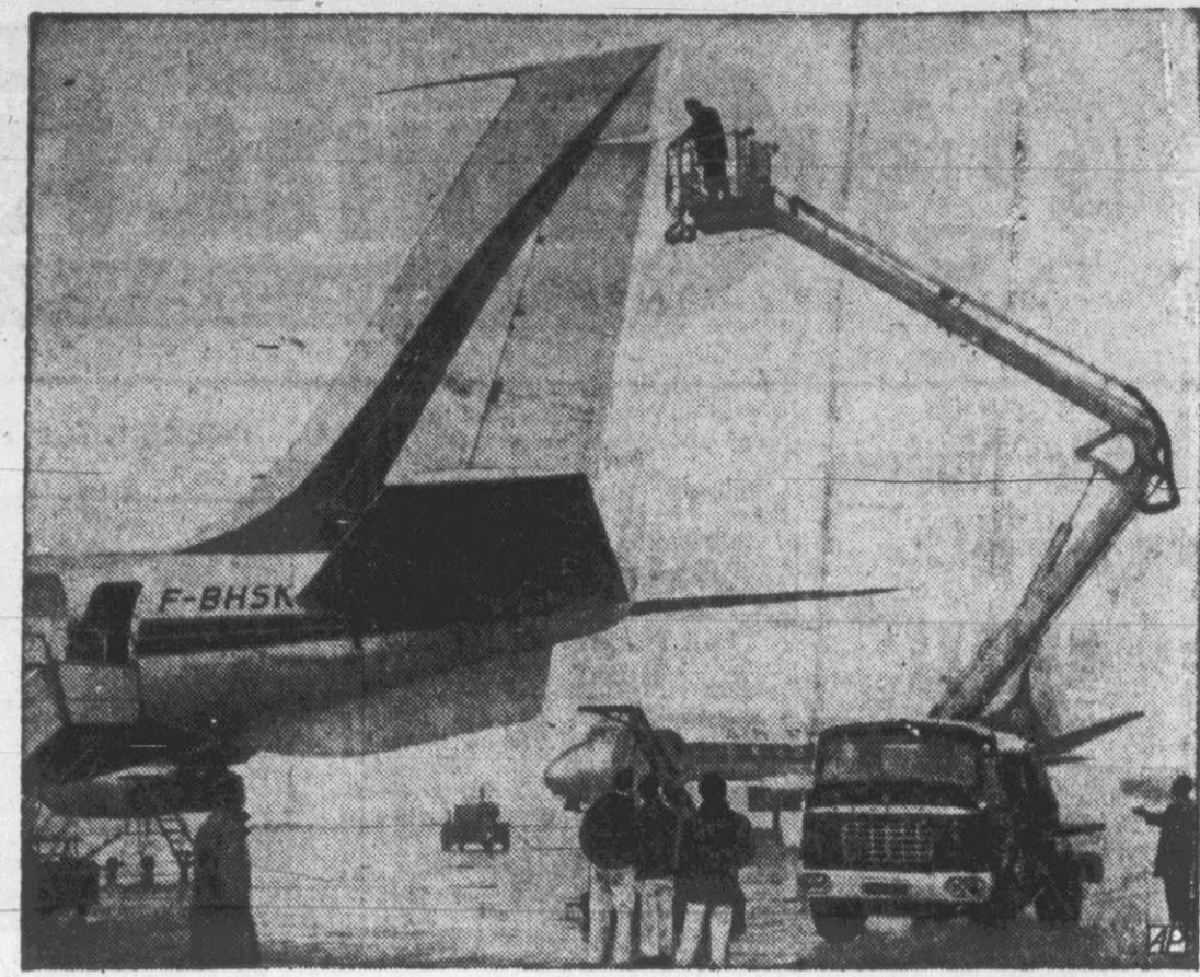
CLEARED FOR FLIGHT —A workman on platform of elbow-jointed hoist sprays alcohol on tail of jetliner to de-ice the craft prior to takeoff from Orly Airport, Paris. All planes leaving the field are de-iced in this manner during current cold spell.
