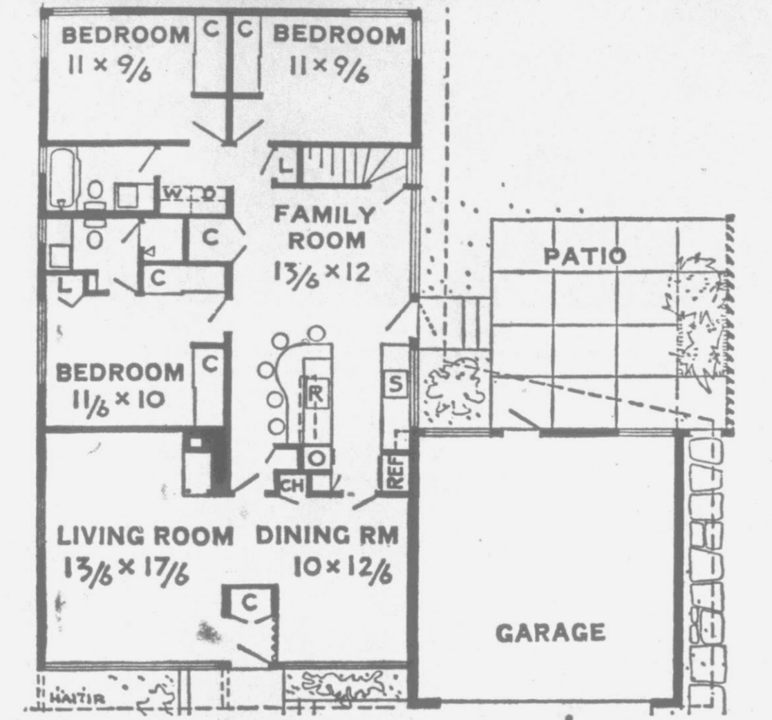
NARROW DESIGN: This three bedroom ranch type home is especially designed for a narrow lot. It is 50 feet deep with a 48-foot frontage, including an attached garage and a patio. A centrally located kitchen is handy to both dining room and patio for indoor and outdoor eating. The architect is Jan Reiner, Box 96, New Port Richey, Fla. and the plan is HA 171R.
