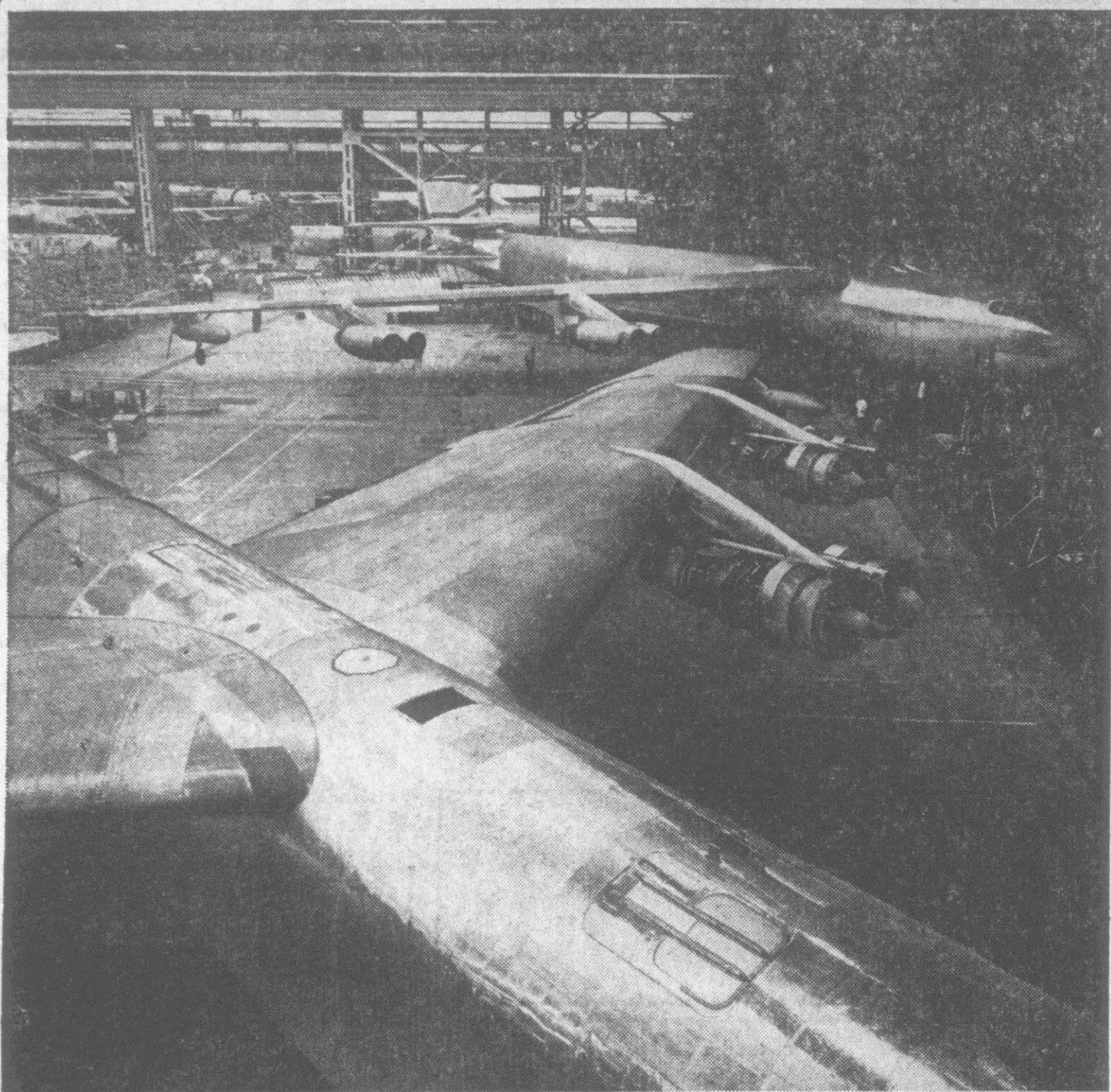
As last B52G moves out into the night, first of B52Hs (foreground) moves in to take its place. The "G" has a plus-9,000 mile range, carries nuclear bombs plus two Hound Dog missiles that can go more than 500 miles farther at supersonic speed. The "H" will go faster, higher, farther—and carry Skybolt missiles, solid fuel ballistic missiles credited with a 1,000 mile range at 3,500 miles per hour.
