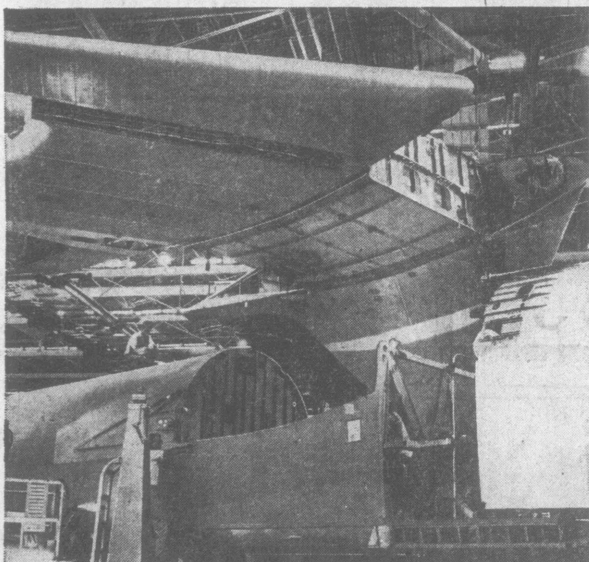
2. Wing section, swung from electric cranes on overhead tracks, moves into place. Workmen are ready to secure wing as it drops into place.
