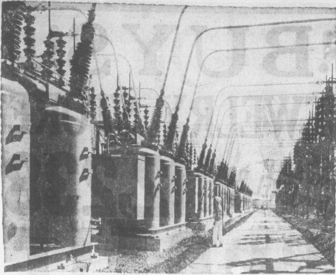
POWER SWITCHYARD—Oil circuit breakers, left, and disconnect switches flank road in main generating plant of Niagara Power Project at Niagara Falls, N.Y. The plant is heart of the system that will have an installed capacity of 2,190,000 kilowatts.
