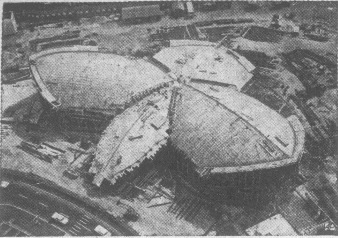
VIEW FROM ABOVE — Wooden forms are in place awaiting the pouring of concrete for the 6,000-ton roof of the new TWA passenger terminal at New York's Idlewild airport. The terminal, to be ready in 1961, is designed to look like a big white bird from the air.
