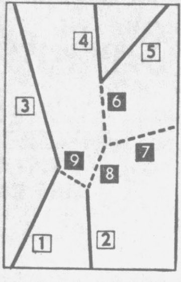
ATOMIC TRACINGS—Particles from the exploding nucleus of an atom trace hetero-skelter patterns on a photographic plate (left). Visible particles (also shown as solid lines on chart) are (1) positive pi meson, (2) K negative, (3) negative pi meson, (4) proton, (5) negative pi meson. Particles not visible on the plate because they have no electrical charge (dotted lines on chart) are (6) lambda neutral, (7) neutral pi meson, (8) XI neutral, (9) K neutral.
