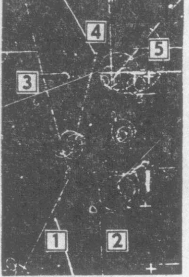
ATOMIC TRACINGS—Particles from the exploding nucleus of an atom trace hetero-skelter patterns on a photographic plate (left). Visible particles (also shown as solid lines on chart) are (1) positive pi meson, (2) K negative, (3) negative pi meson, (4) proton, (5) negative pi meson. Particles not visible on the plate because they have no electrical charge (dotted lines on chart) are (6) lambda neutral, (7) neutral pi meson, (8) XI neutral, (9) K neutral.
