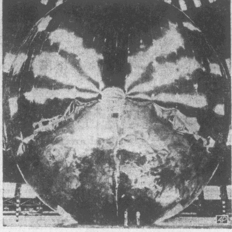
Men appear as midges in front of the 100-foot diameter plastic balloon of the type rocketed into orbit as scientists at Cape Canaveral, Fla. took another step toward establishing a worldwide radio communications system. The balloon rode into space in the nose of a three-stage Thor-Delta rocket. Radio signals will bounce off the aluminum coated balloon as it orbits 1,000 miles above the earth. Photo was made during a recent inflation test. (AP Wirephoto)
