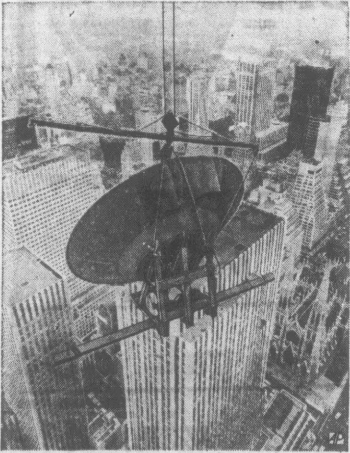
HIGH PERCH—A parabolic reflector, part of New York's weather bureau storm detection radar network, is hoisted to station on 70th floor roof of the RCA Building.
