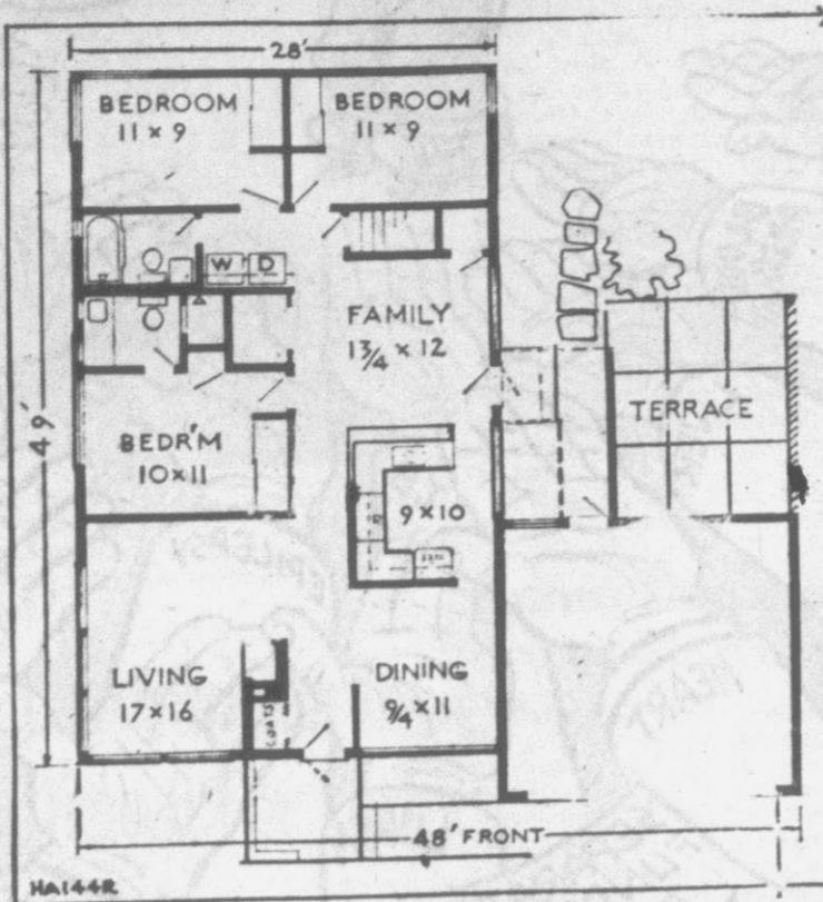
NARROW RANCH: This seven-room ranch can be built on a lot with 75-foot frontage (two-car garage) or 60-foot lot with one-car garage. Vertical redwood siding dresses up exterior. Features are raised corner fireplace in living room, centrally located U-kitchen, two baths, family room and washer-dryer area. The house has 1,248 square feet of floor space and the design, HA144R, is by Architect Jan Reiner, Post Office Box 96, New Port Richey, Fla.
