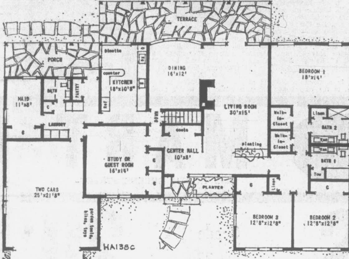
DREAM RANCH: This ranch is luxury unlimited; 2,680 square feet of well-planned comfort. The design features three large bedrooms (one 18x14), study, living room, dining room, kitchen with dinette and maid's room with separate bath. The house is 48 feet deep and 80 feet wide. Architect is Lester Cohen, Room 75, 117 W. 48th St., New York, N. Y., and the plan is HA138C.
