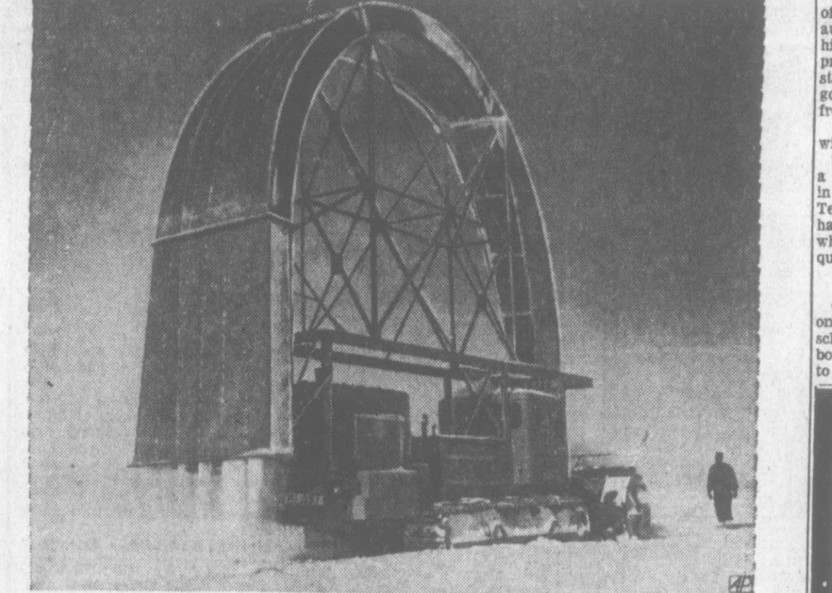
SURFACING THE SNOW — A giant snowblast machine undergoes test by the U. S. Army Corps of Engineers in the frozen Arctic. Machine compacts gathered snow and re-deposits it into a hard, smooth surface—in this case a possible plane runway.
