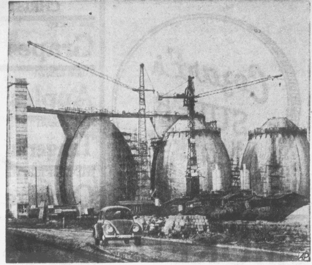
EGG-SHAPED PURIFIERS — These three giant "eggs" housing filter systems were built in Hamburg, West Germany, to purify industrial waste waters going into the Elbe river. Bathing had been forbidden in Elbe because of water pollution.
