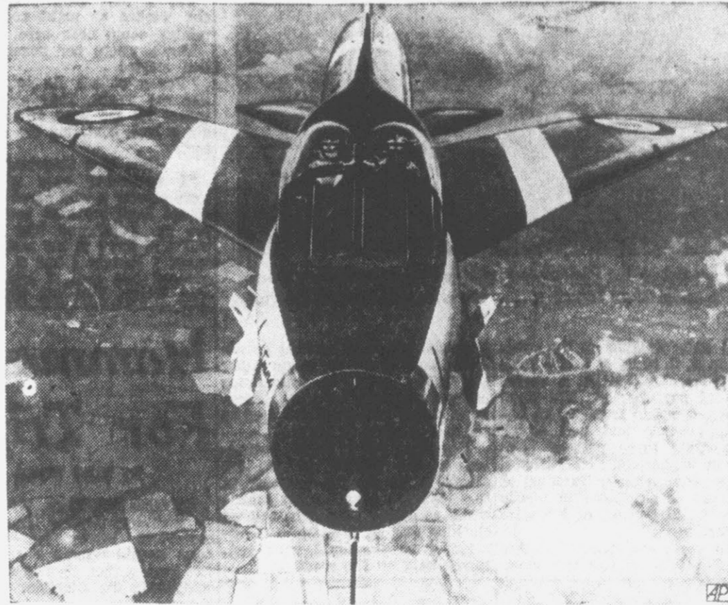
BUZZING ON A HIGH —The British Electric P-11 Lightning two-seat trainer looks like a huge bug in flight over England. Two Firestreak guided missiles on either side of fuselage are part of the armament system of the RAF all-weather jet fighter.
