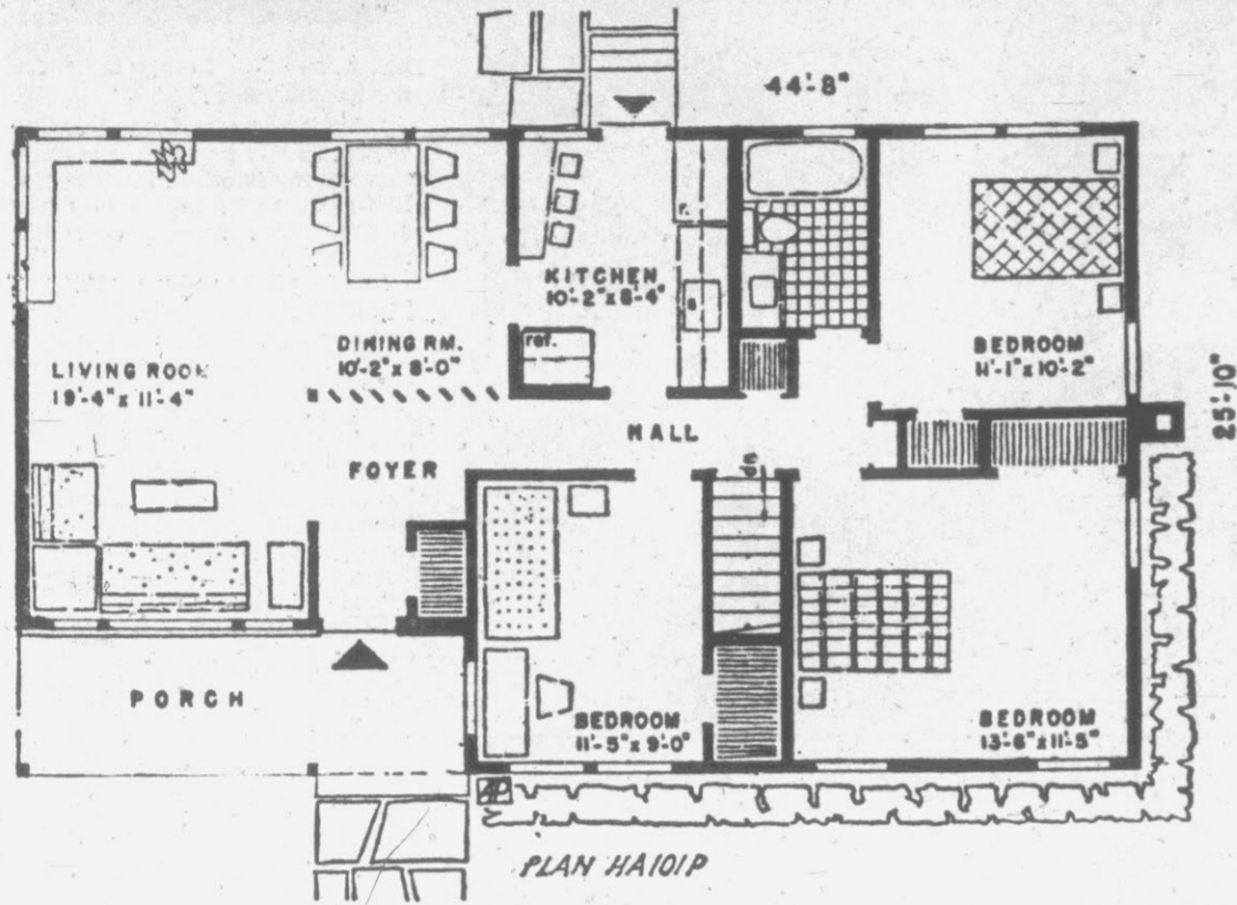
PRACTICAL PACKAGE: In only 1,048 square feet of floor space, this ranch achieves a maximum of livability—three bedrooms with cross ventilation, an almost-20 ft. living room, eating space in the kitchen, and a dining area. A garage can be added to the left side of the living room. It is Plan HA101P, by Architect Samuel Paul, 89-51 164 St., Jamaica, N. Y.
